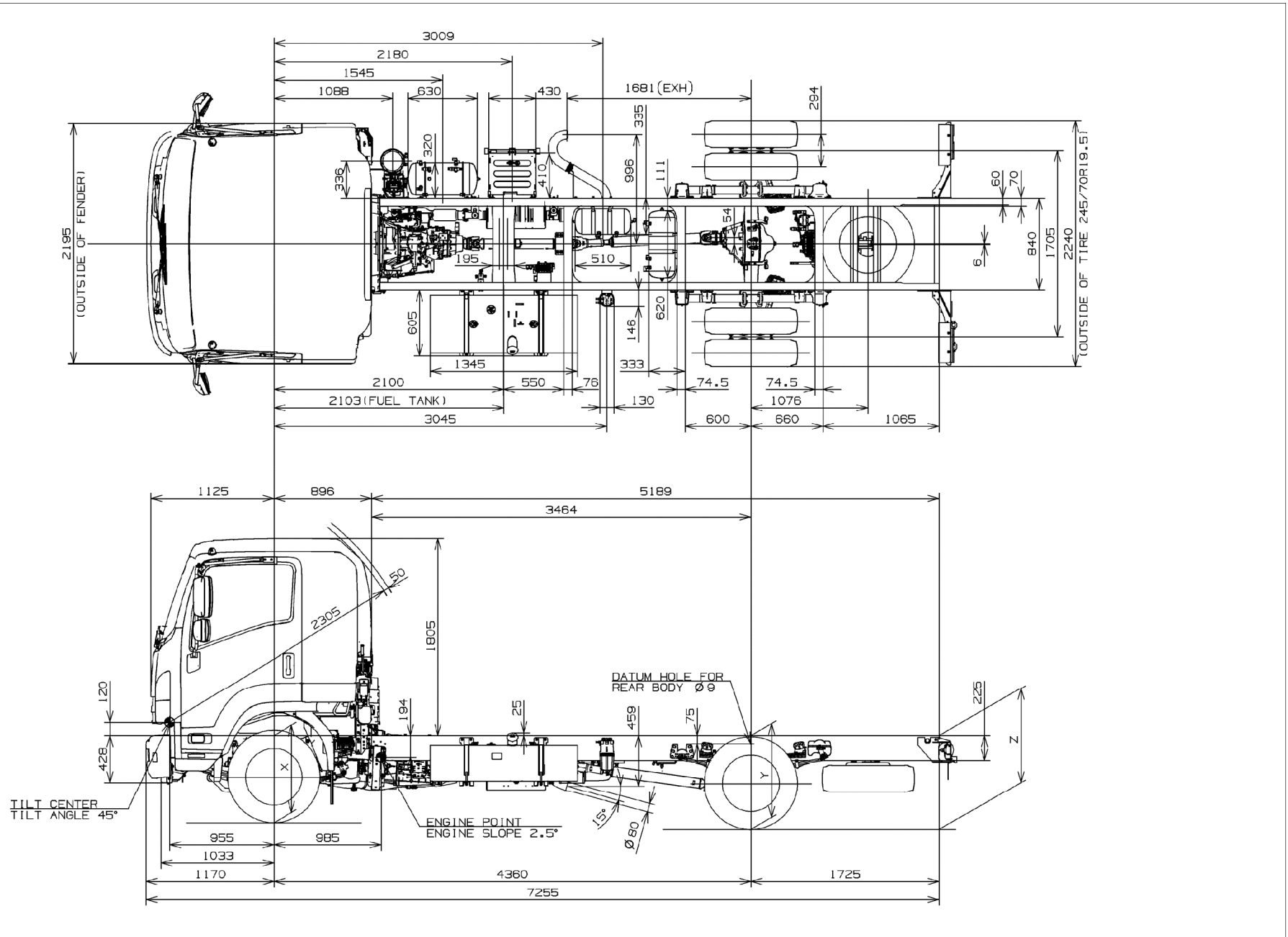
Fig. 9-1-1 Cab Chassis Drawing FSR34UL-LCUN
