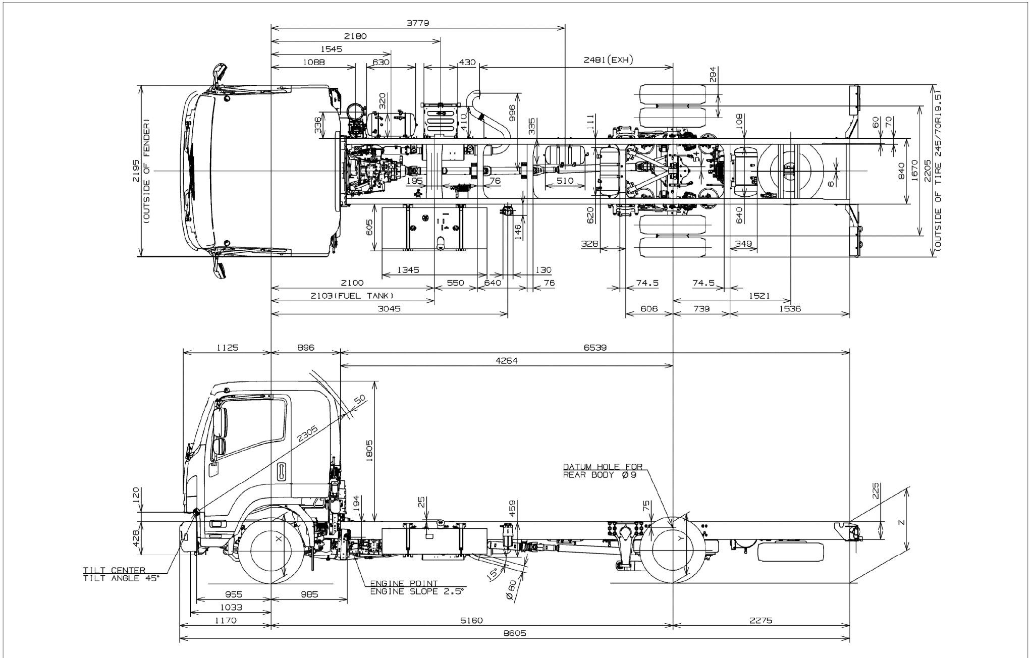
Fig. 9-1-5 Cab Chassis Drawing FSR34VL-PCUN
