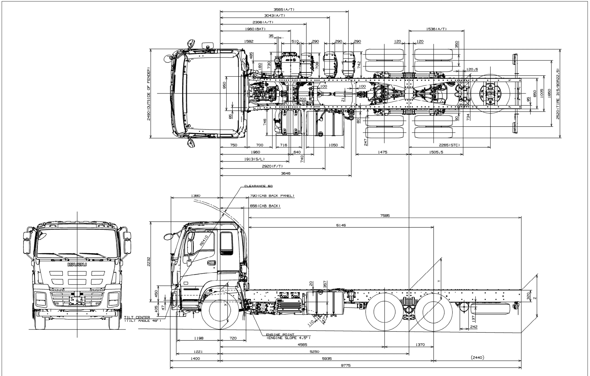
Fig. 9-1-6 Cab Chassis Drawing CYZ52QLX3T17
